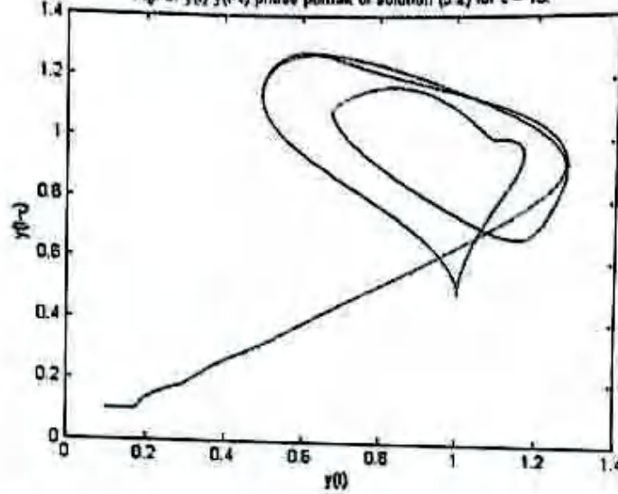
Fig. 9: Comparison of solutions (5.2) for \tau = 20 .
