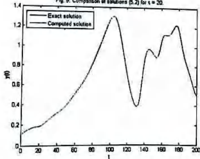
Fig. 9: Comparison of solutions (5.2) for \tau = 20 .
