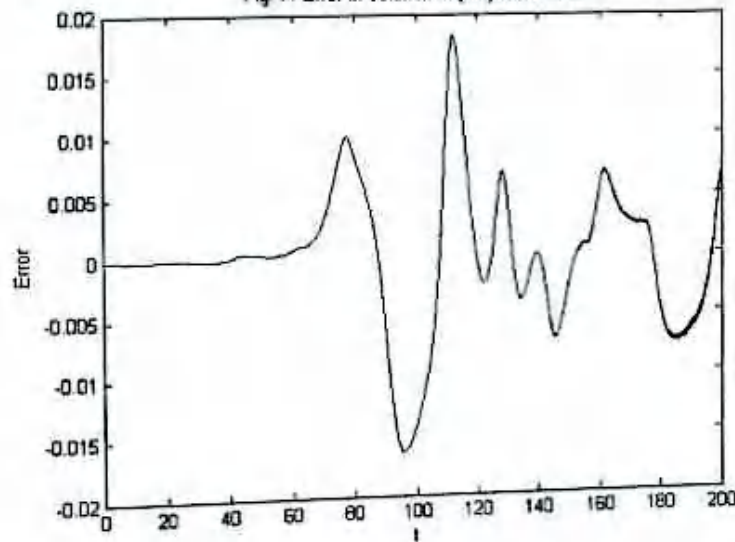
Fig 7: Error in solution of (5.2) for \tau = 15
